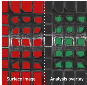
ASTM Class 1, ISO Class 4, Undamaged area: 35.5%
