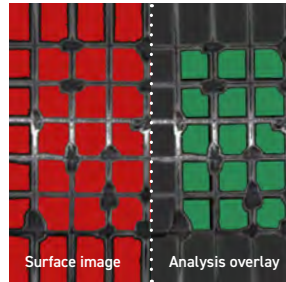
ASTM Class 2, ISO Class 3, Undamaged area: 79.7%
