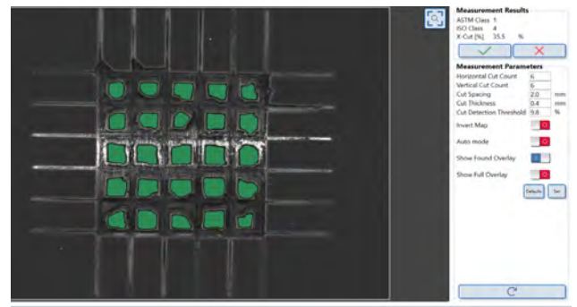
Cross-cut percentage reported directly on screen with ASTM / ISO class
