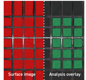
ASTM Class 4, ISO Class 1, Undamaged area: 98.5%
