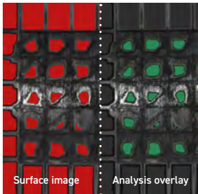
ASTM Class 0, ISO Class 5, Undamaged area: 16.5%
