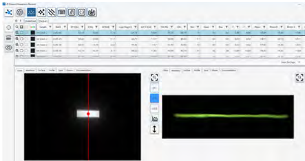
Surface brilliance module showing numeric results, measurement images and graph.
